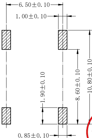
SUGGESTED PCB LAYOUT (COMPONENT SIDE)
